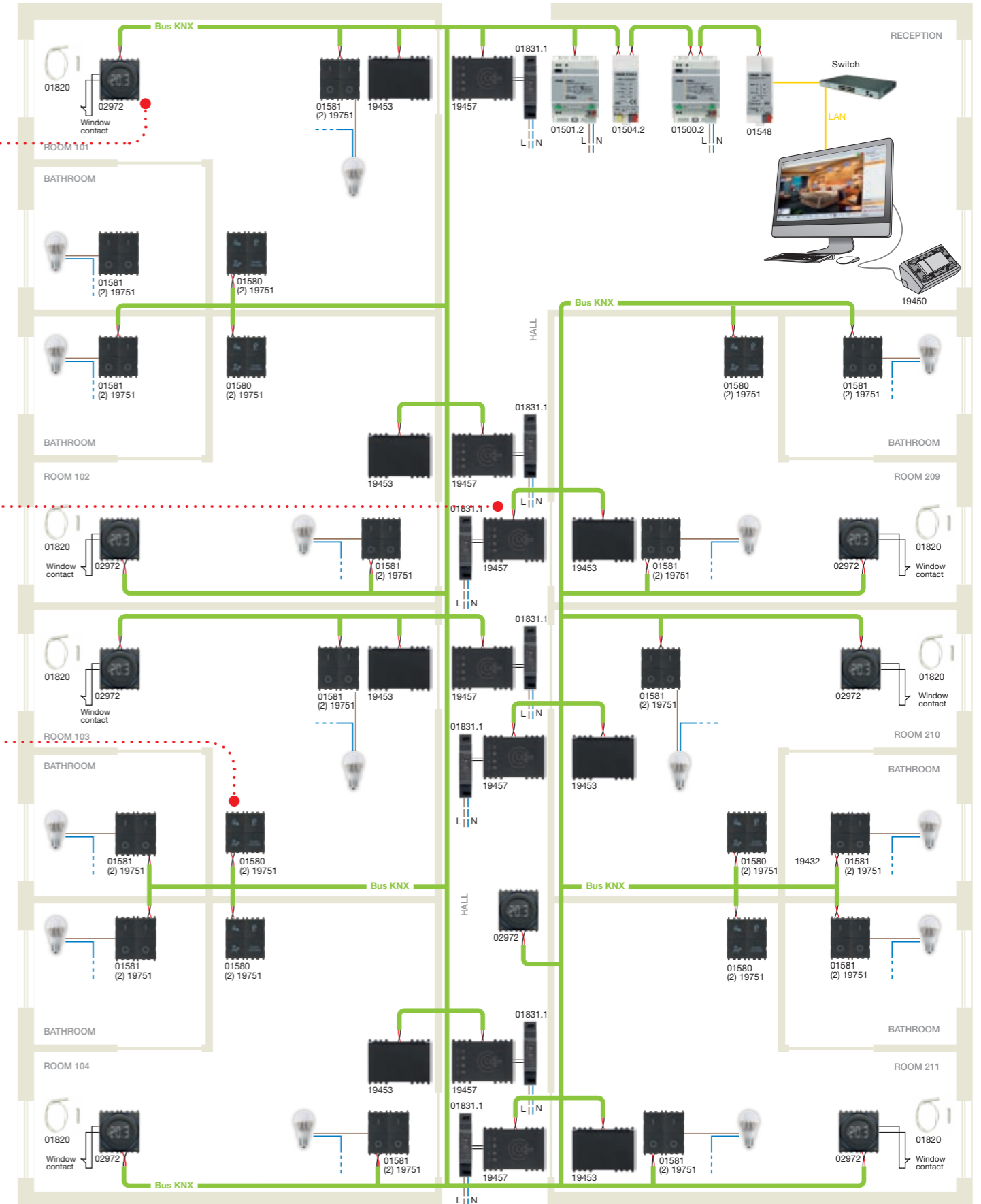
— KNX Bus — Probes connection — Power supply 230 V- — Wired connection — LAN connection — Auxiliary power supply 12 V
