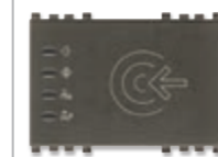
19457.M Transponder card reader for installation outside rooms, KNX standard, 2 NO 4 A 24 V~ relay outputs, 2 inputs, power supply 12-24 V~ 50/60 Hz and 12-24 Vdc (SELV), Metal - 3 modules. Supplied without transponder card. Depth: 37 mm
